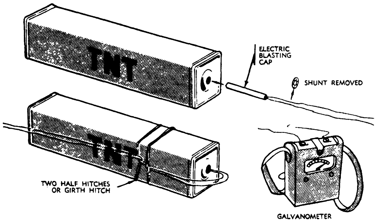
Figure 2-23. Electric priming of demolition block without priming adapter.
