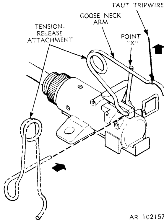
Figure 2-44. Installing tension release attachment.
