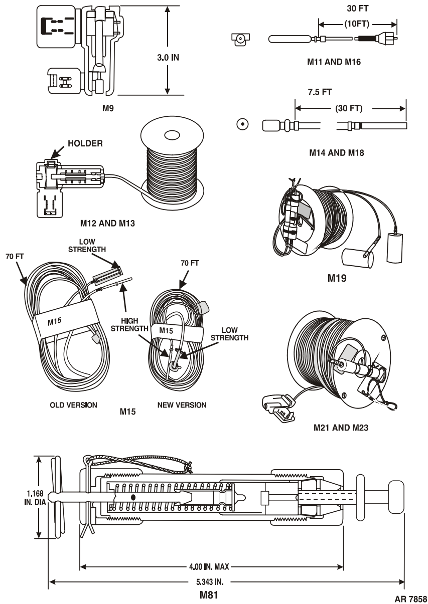
Figure 1-11.1 - Modernized Demolition Initiators (MDI) Components.
