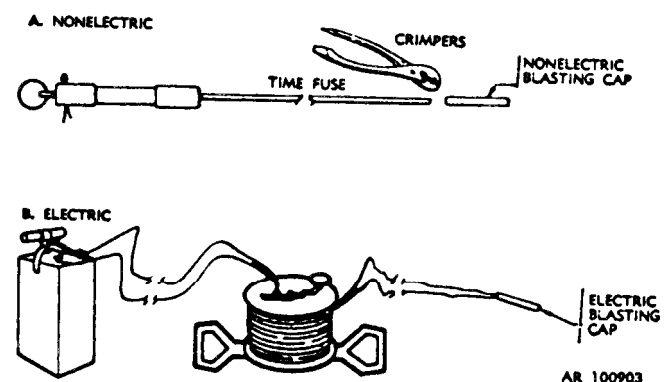
Figure 2-1. Initiation systems.
